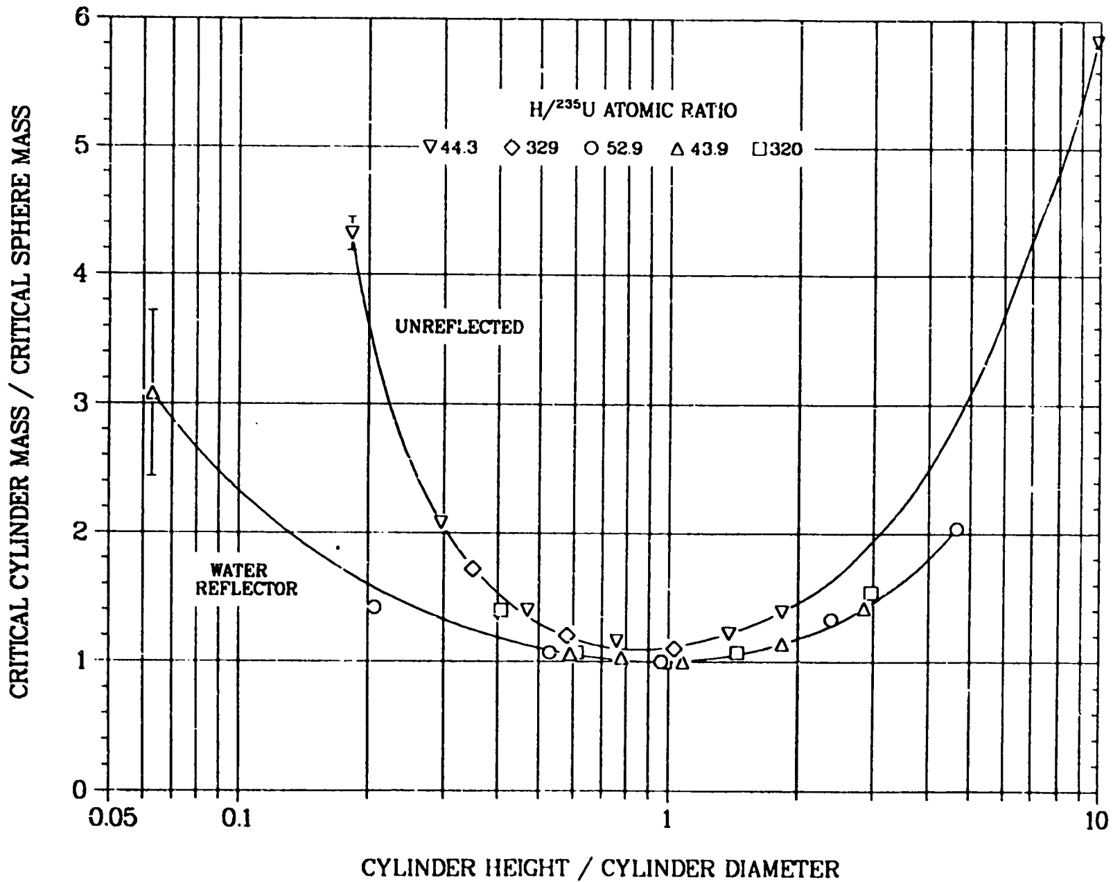
Figure 4. The ratio of cylindrical to spherical masses of U(93)O 2 F 2 solutions, unreflected and with water reflector, as a function of cylinder height to cylinder diameter ratio.
