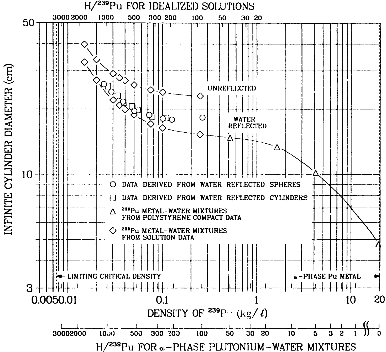
Figure 14. Estimated critical diameters of infinitely long cylinders of homogeneous water-moderated ^{239}\text{Pu} . The points suggesting an intermediate curve apply to water-reflecting \text{Pu}(\text{NO}_3)_4 solutions with 1 N \text{HNO}_3 and 3.1% ^{240}\text{Pu} content of the plutonium. (From LA-10860-MS, Figure 33).
