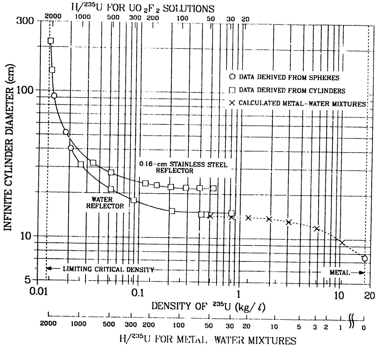
Figure 13. Estimated critical diameters of infinitely long cylinders of homogenous water-moderated U(93.2) spheres. Solution data appear unless indicated otherwise. (From LA-10860-MS, Figure 12).
