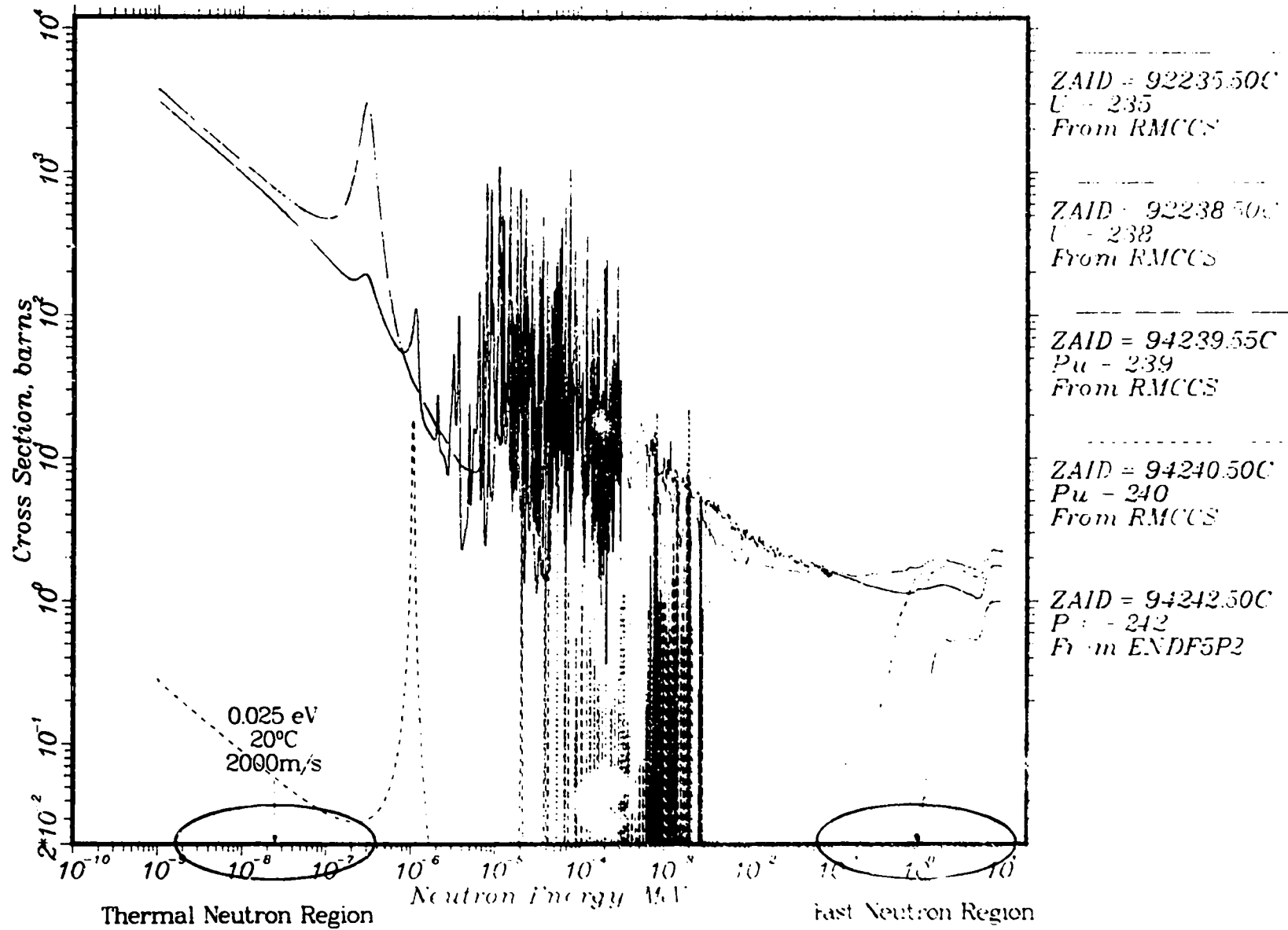
Figure 2. Fission cross sections for selected isotopes.
