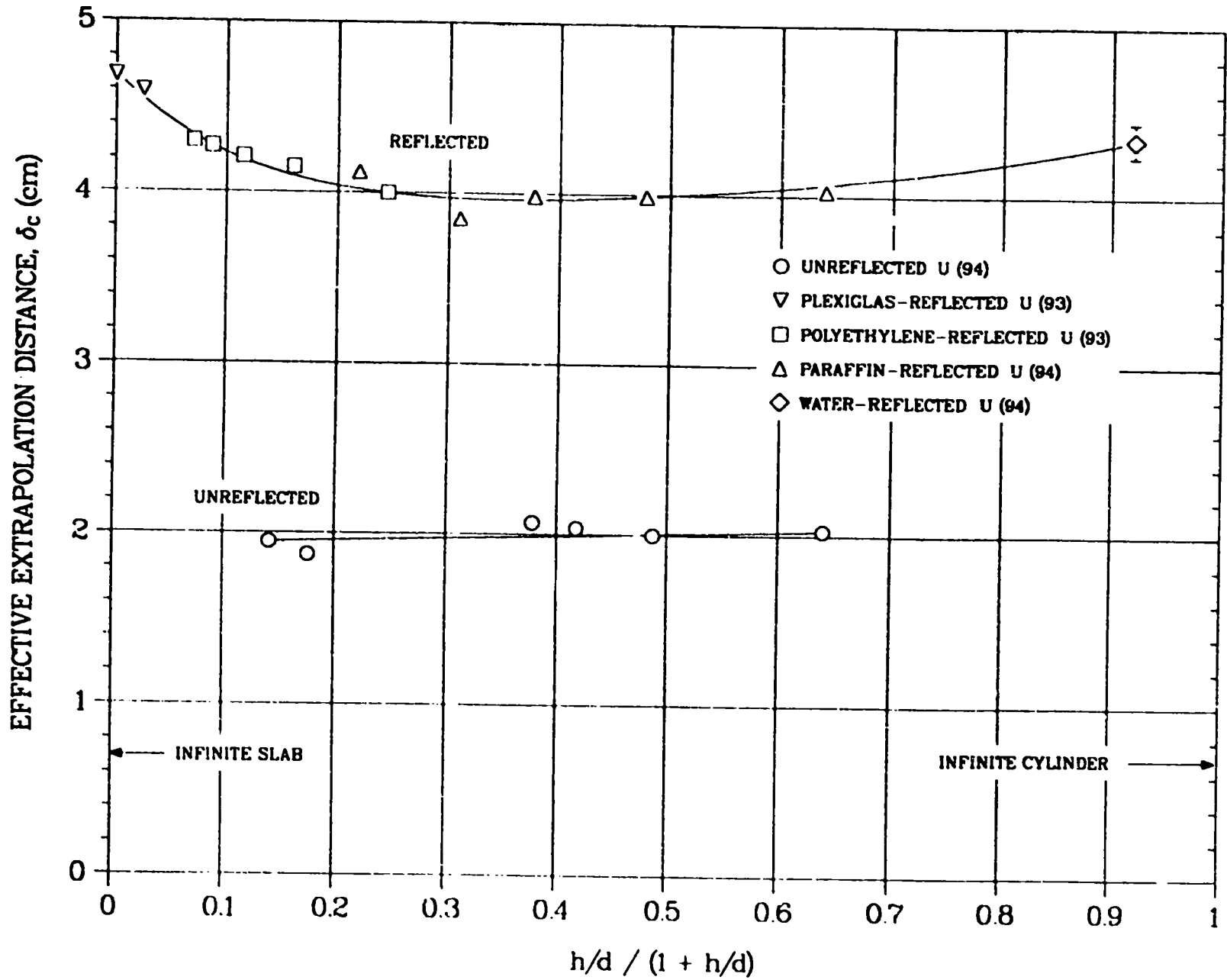
Figure 7. Effective extrapolation distances of U(>90) metal cylinders, unreflected and with hydrogenous reflectors. Cylinder height and diameter are h and d, respectively.
