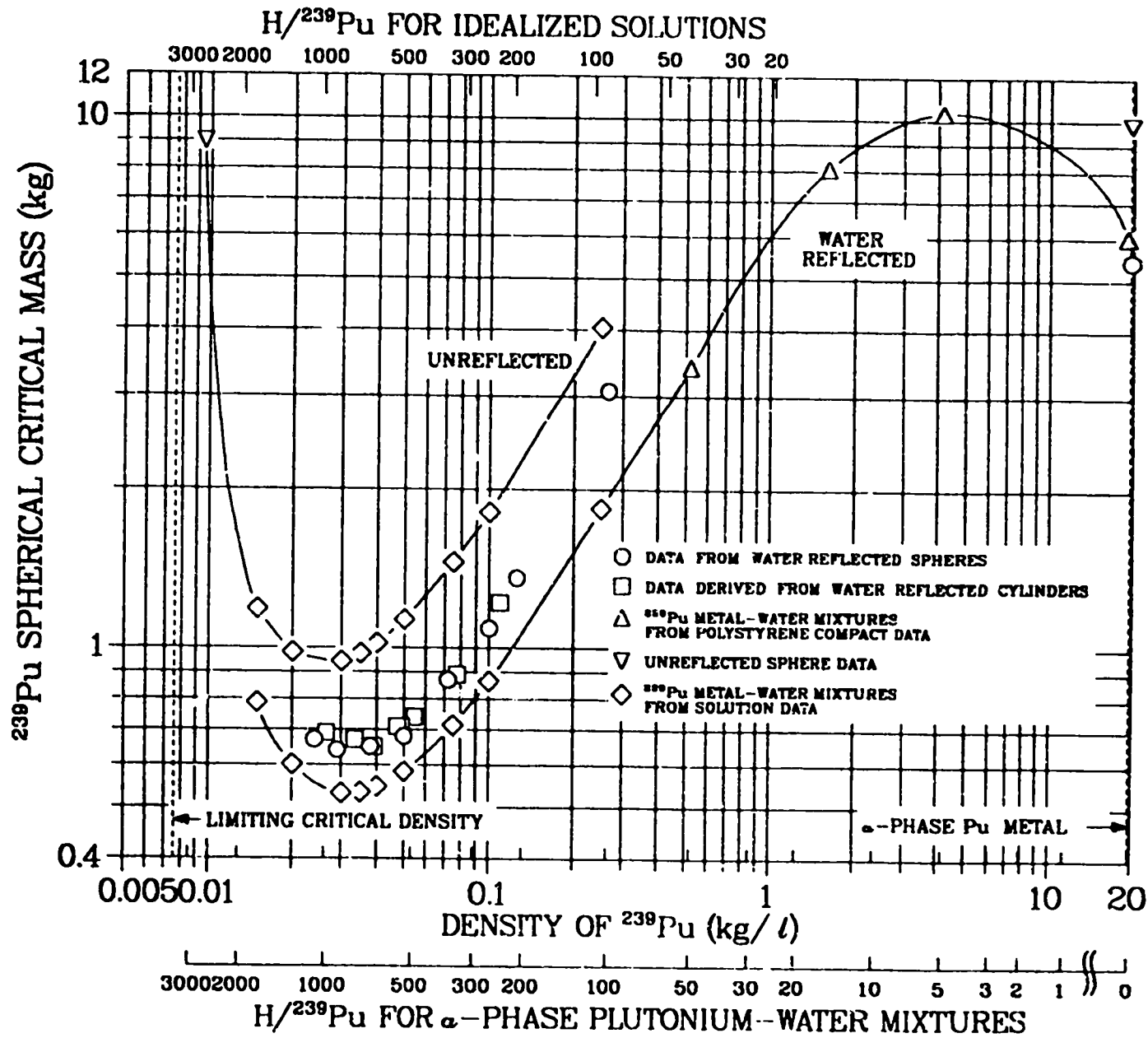
Figure 11. Critical masses of homogeneous water-moderated ^{239}\text{Pu} spheres. The points suggesting an intermediate curve apply to water-reflected \text{Pu}(\text{NO}_3)_4 solutions with 1 N \text{HNO}_3 and 3.1% ^{240}\text{Pu} content of the plutonium. (From LA-10860-MS, Figure 31).
