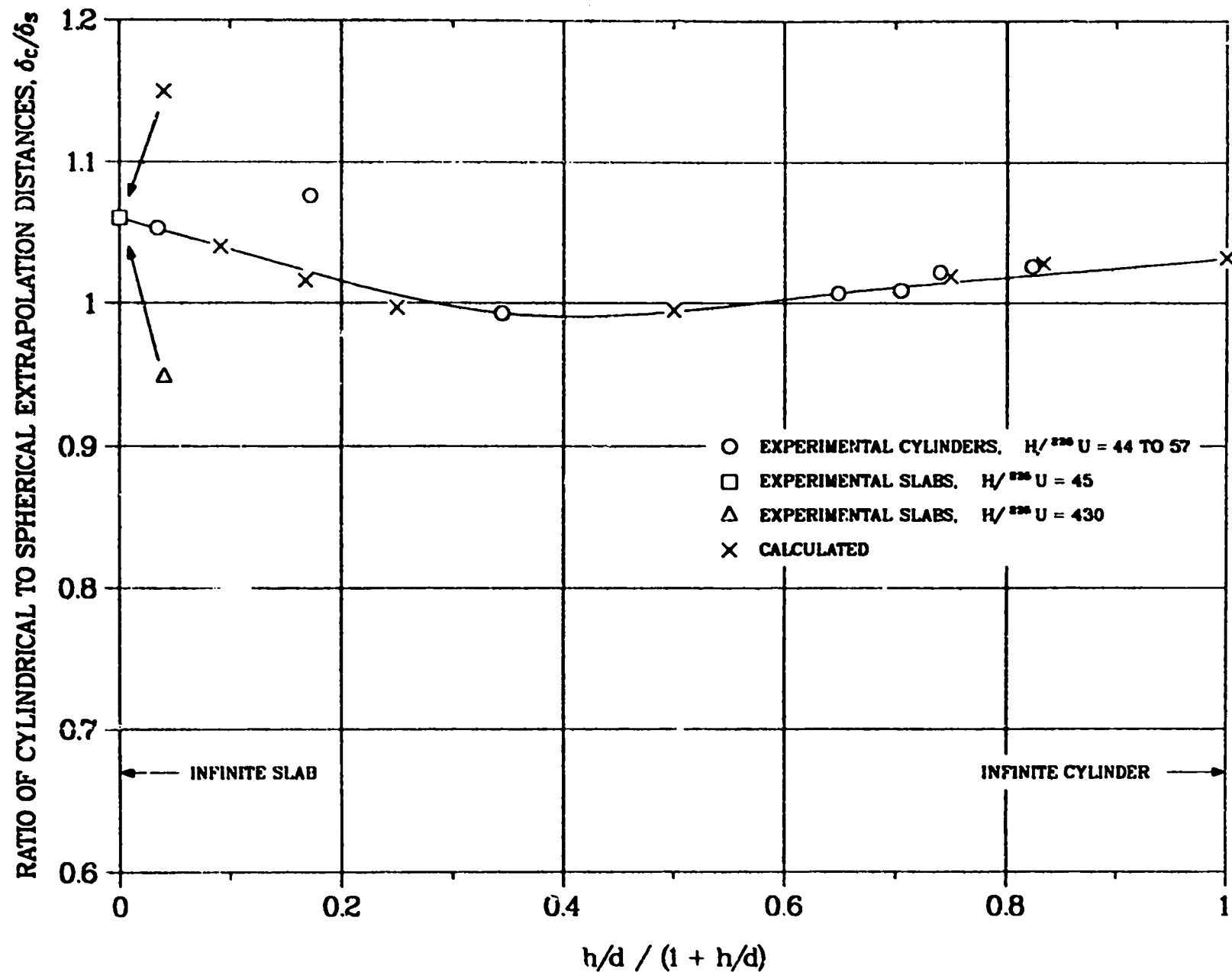
Figure 6. Ratio of extrapolation distance to that of sphere to water-reflected \text{U}(93)\text{O}_{22}\text{F}_4 solutions. Cylinder height and diameter are h and d , respectively.
