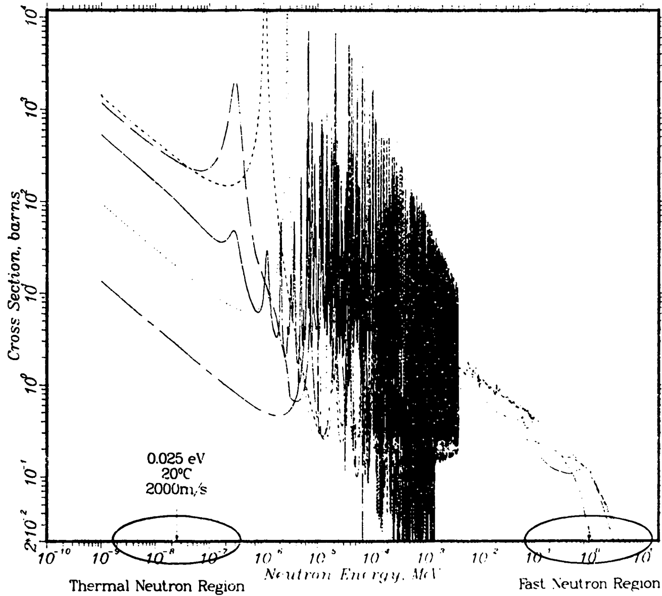
Figure 4. Capture cross sections for selected isotopes.
